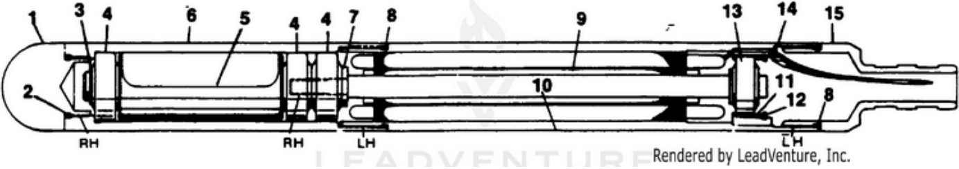
VCH200D 180 Cycle Concrete Vibrator UT-06052 - Exploded View
