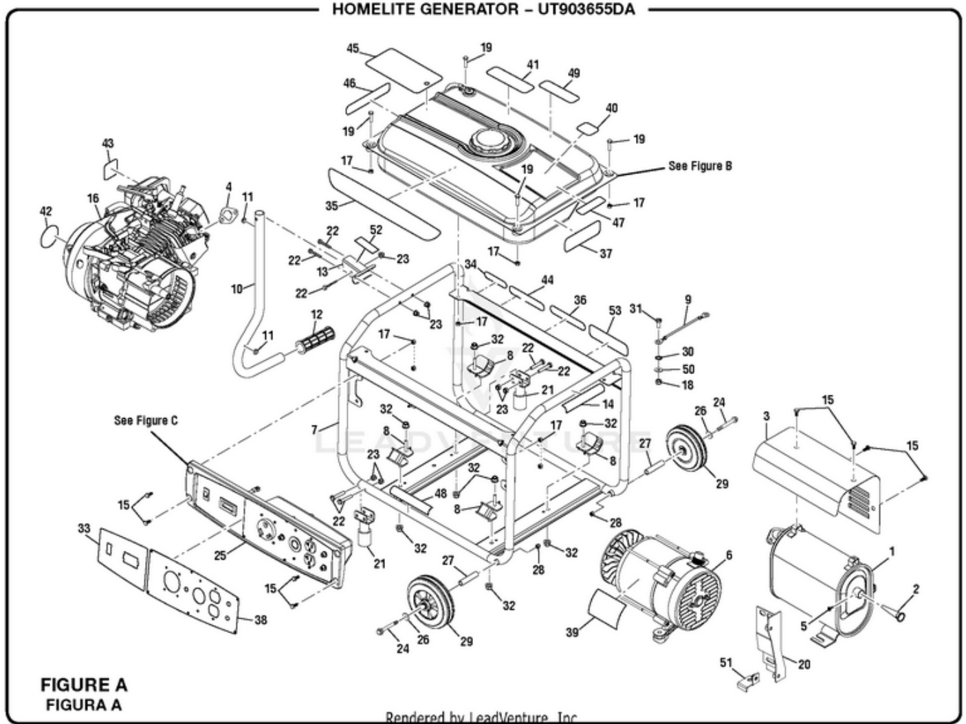
UT903655DA 3650 Watt Generator (990000673) - Figure A
