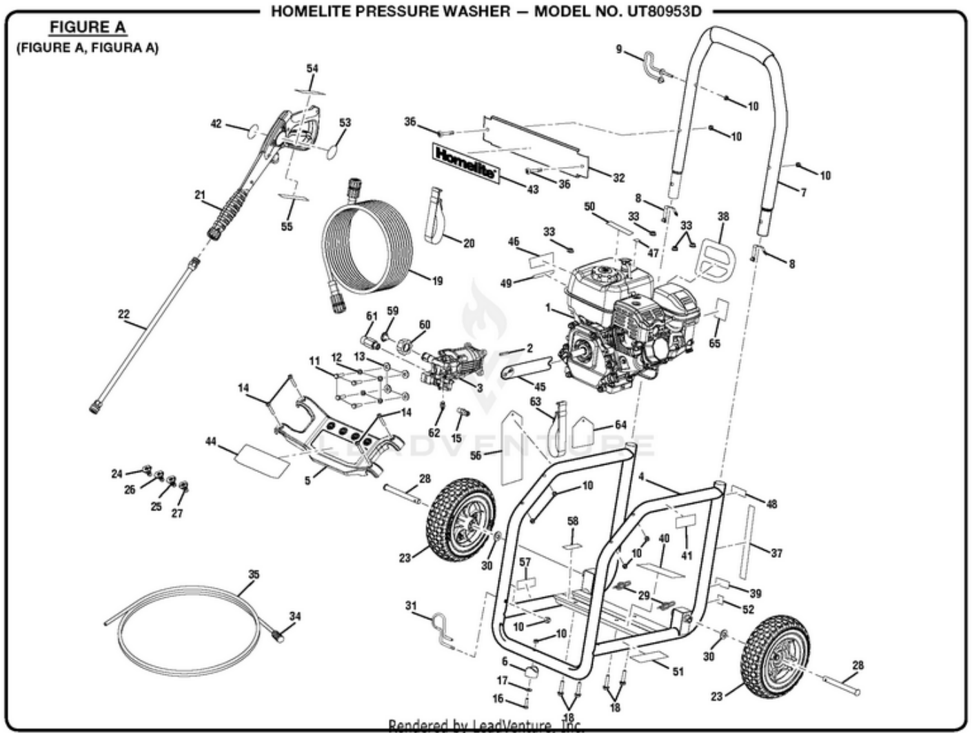
UT80953D Pressure Washer - Figure A
