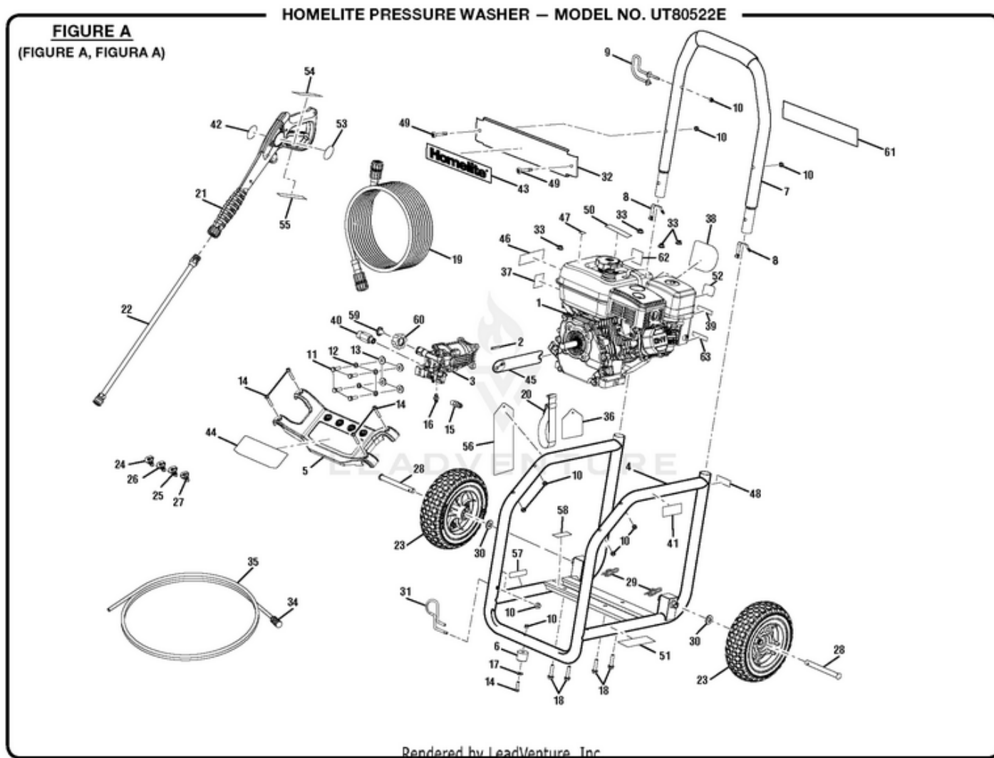
UT80522E Pressure Washer - Figure A
