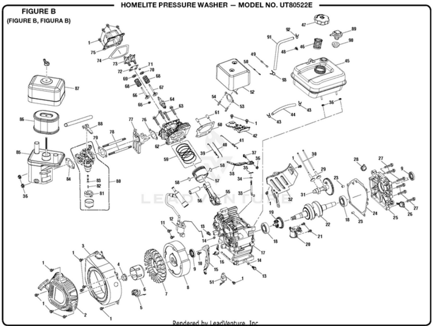
UT80522E Pressure Washer - Figure B
