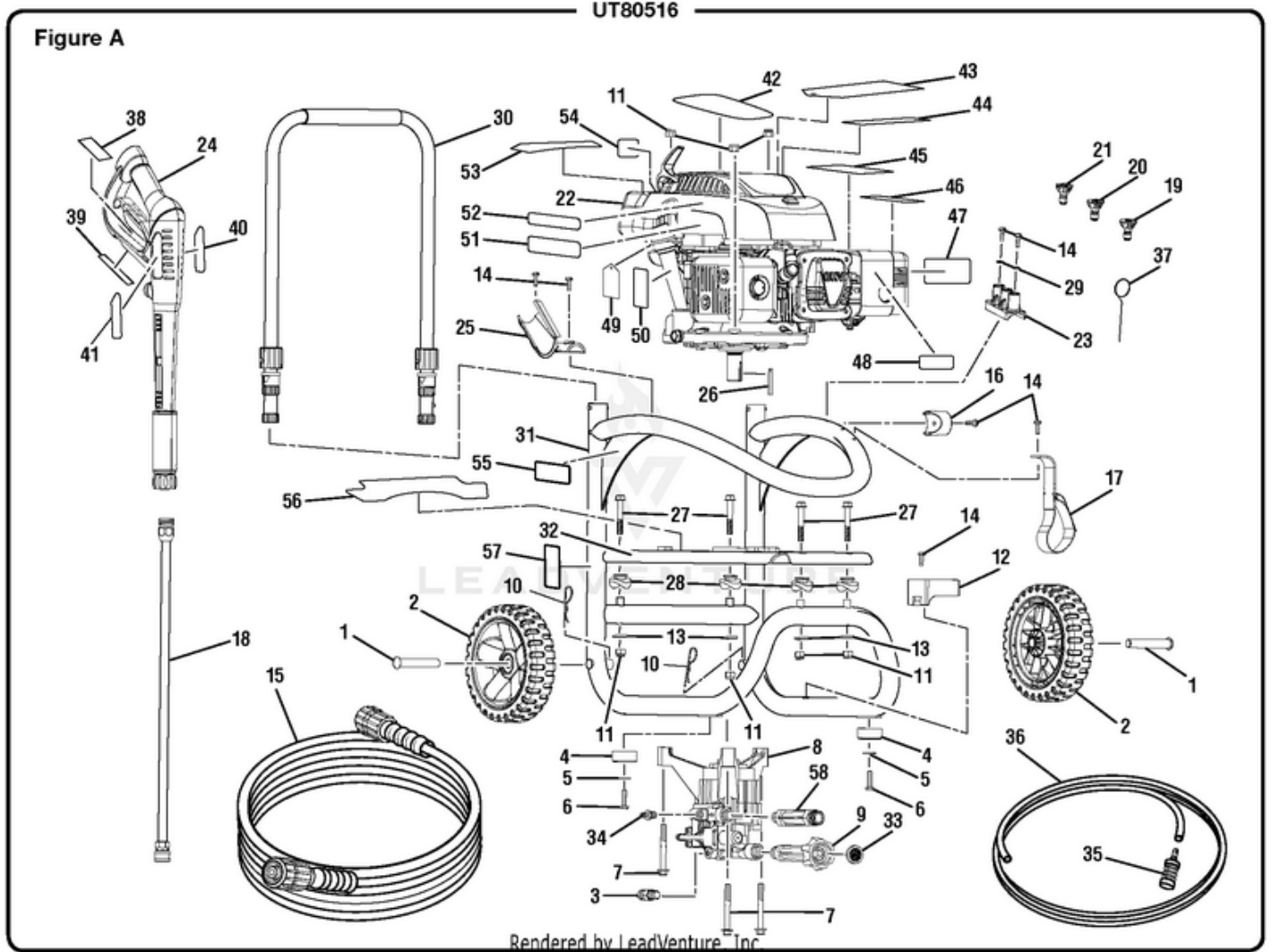
UT80516 2200 PSI Pressure Washer - Figure A
