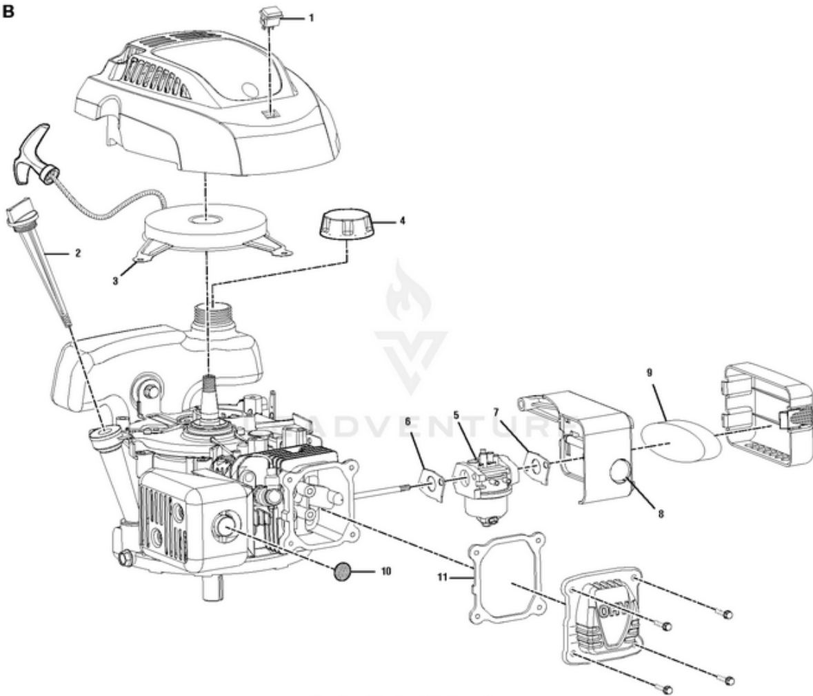
UT80516 2200 PSI Pressure Washer - Figure B
