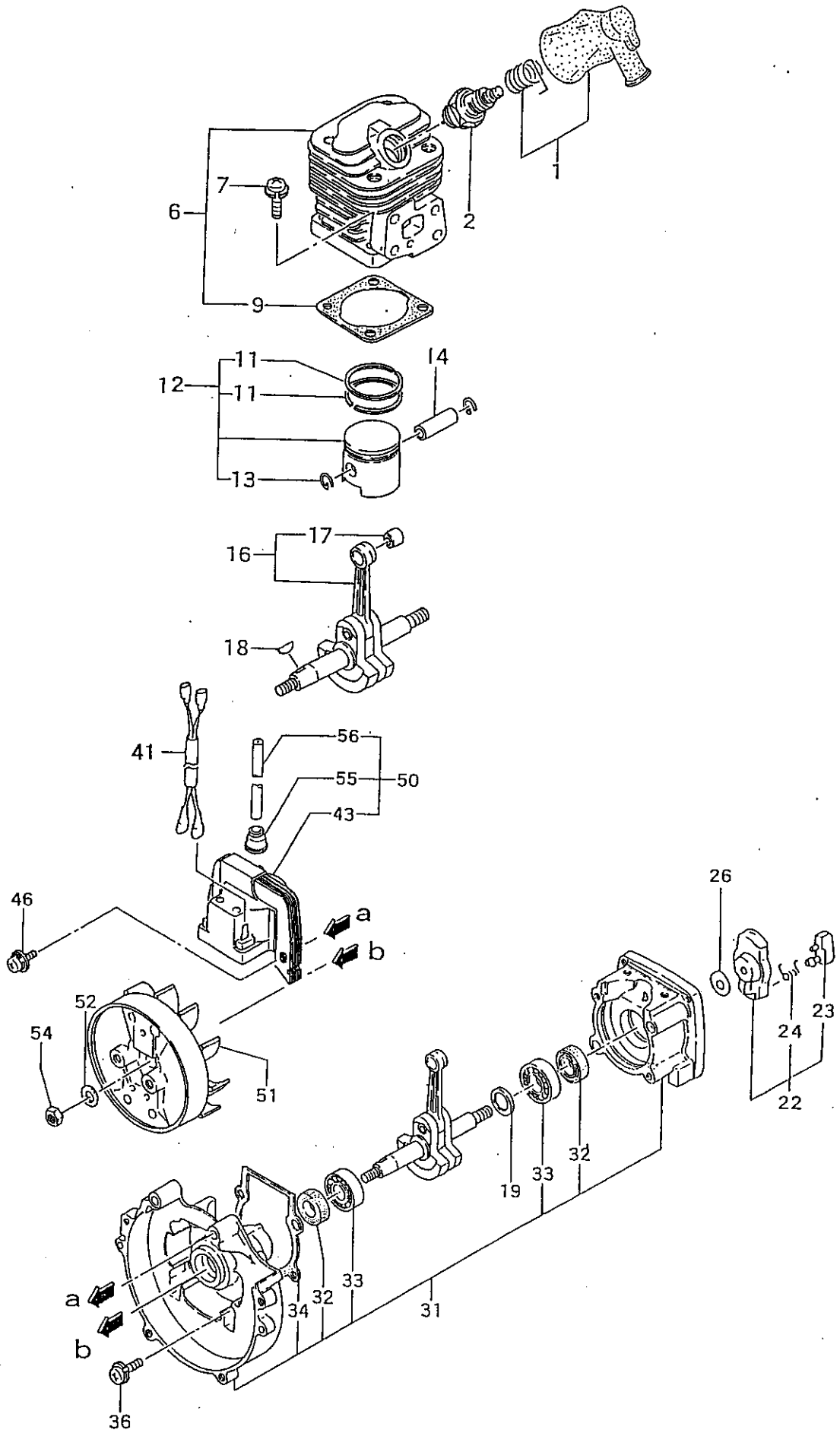
FIG. 1 ENGINE
