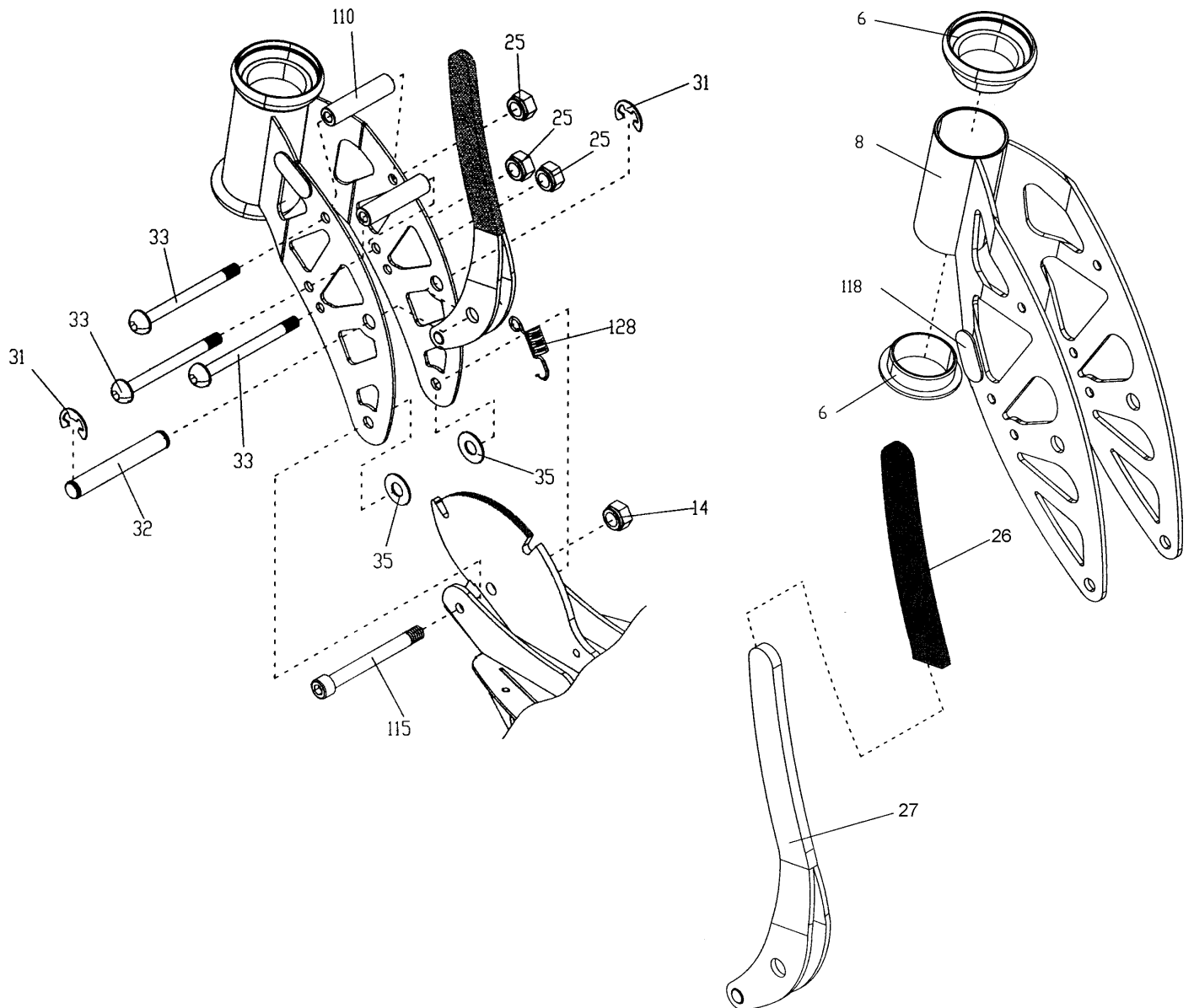
HEAD PIPE & FOLDING HANDLE • FIGURE 2
