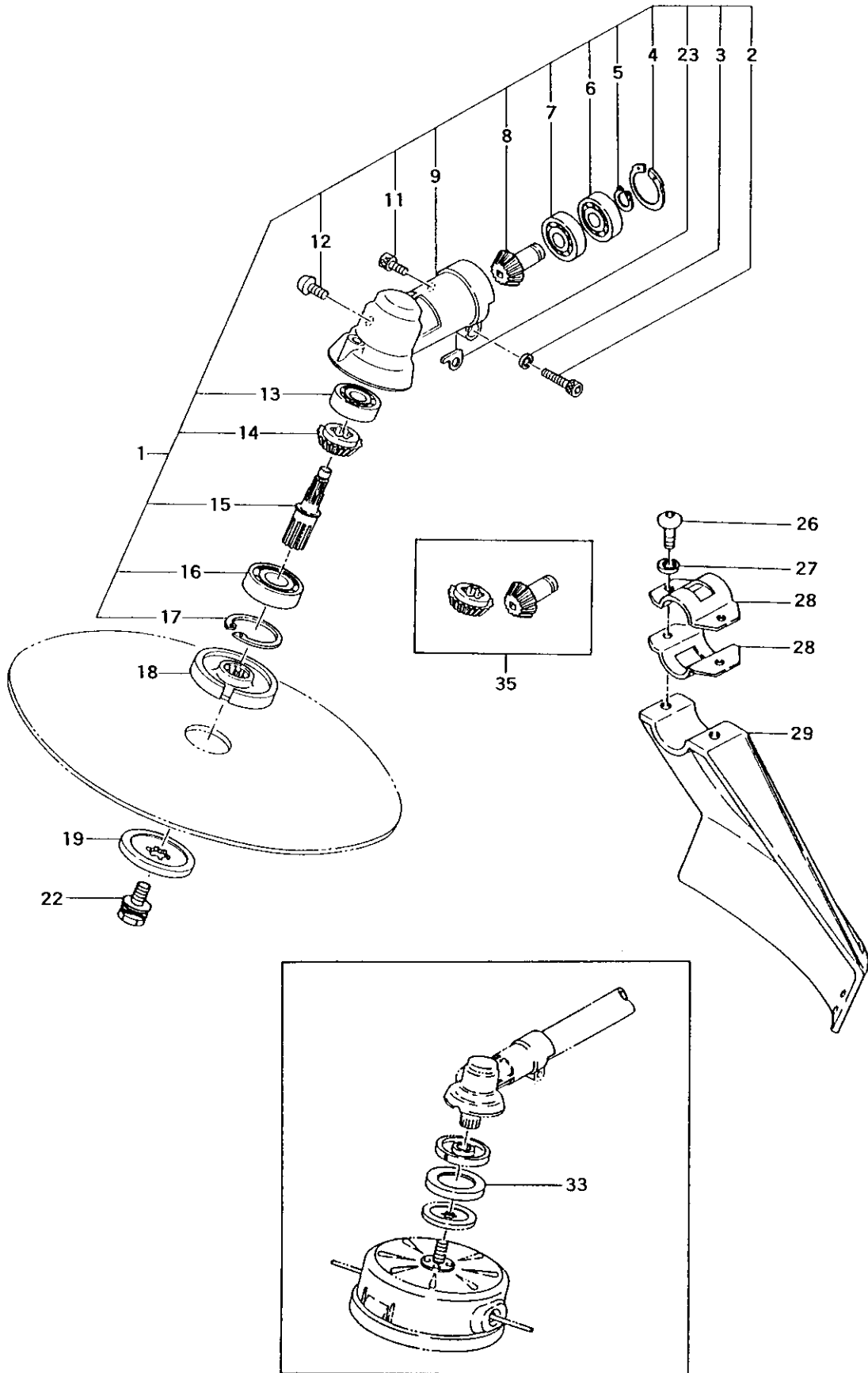
FIG.7 GEAR CASE
