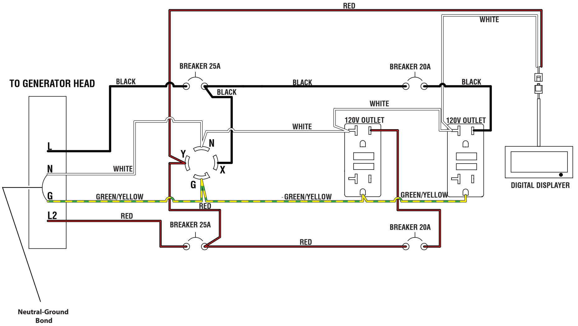
WIRING DIAGRAM
