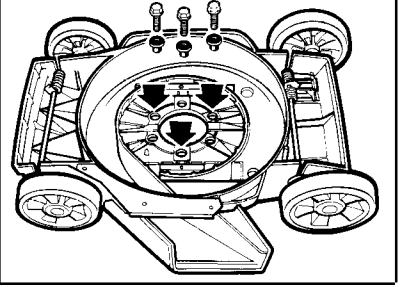
MOTOR MOUNT (Bottom View): Items 53, 54 assembled in 3 locations indicated.
