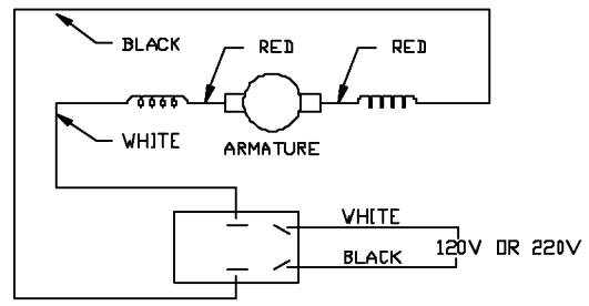
120V OR 220V WIRING DIAGRAM
