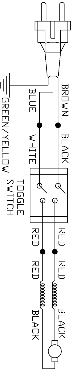
230V WIRING DIAGRAM
