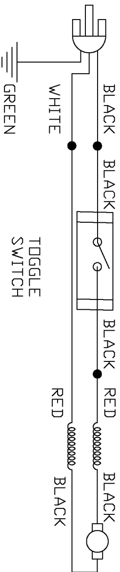
120V WIRING DIAGRAM
