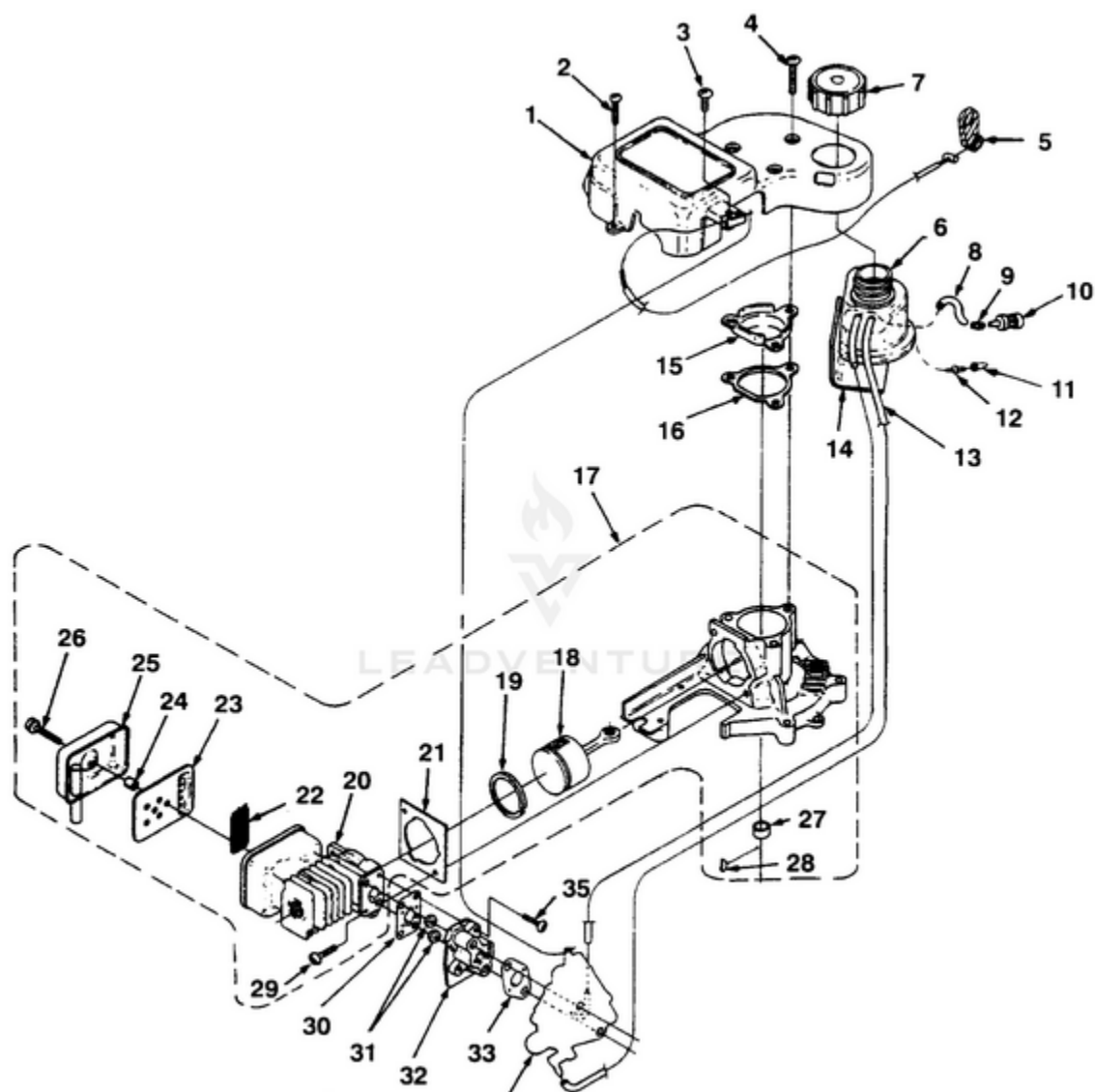
HT19 Hedge Trimmer UT-18023-A - Figure A
