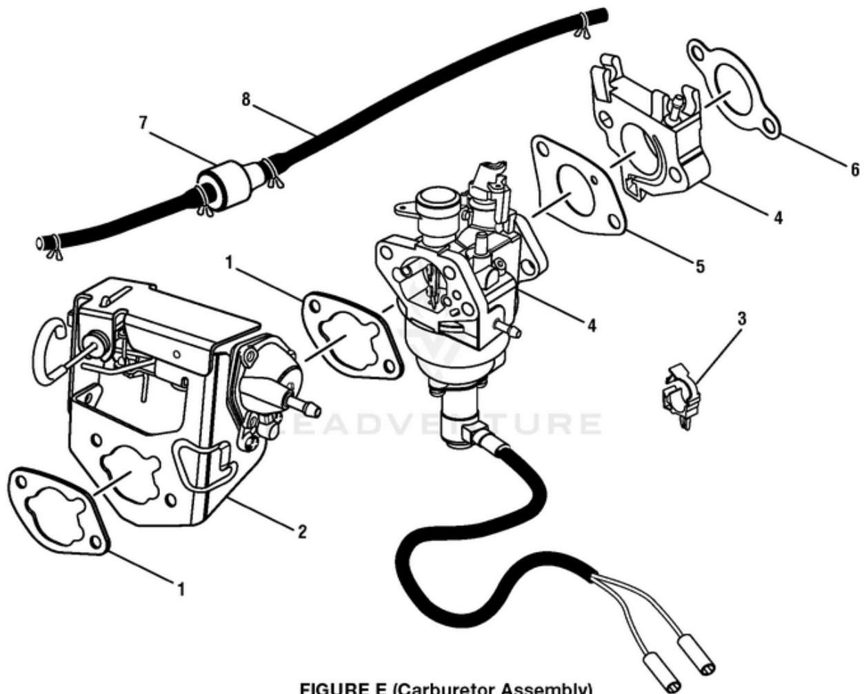
FIGURE E (Carburetor Assembly)
