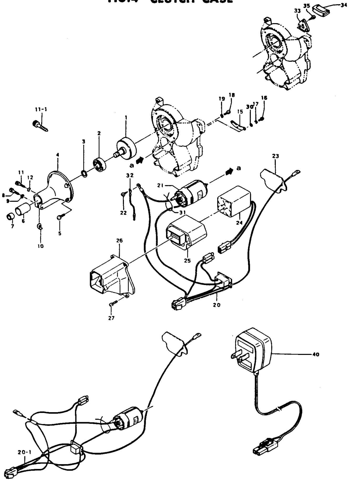
FIG.4 CLUTCH CASE
