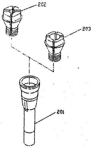
43-800 ROUTER / ADAPTER SPINDLE
