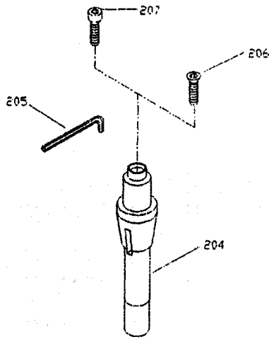
43-809 STUB SPINDLE
