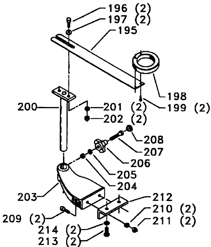
43-359 RING GUARD
