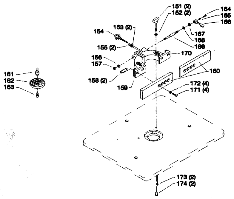
43-158 SHAPER FENCE
