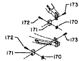
40-603 90° BLADE HOLDER
