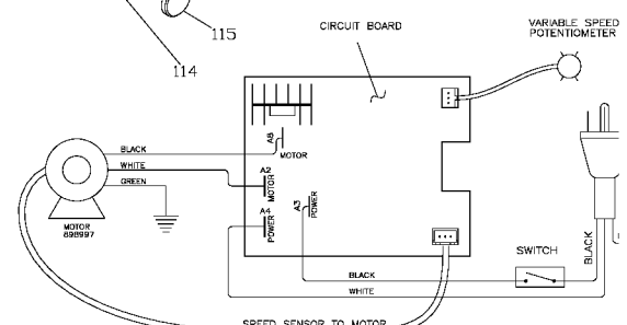
WIRING DIAGRAM 40-670 SCROLL SAW
