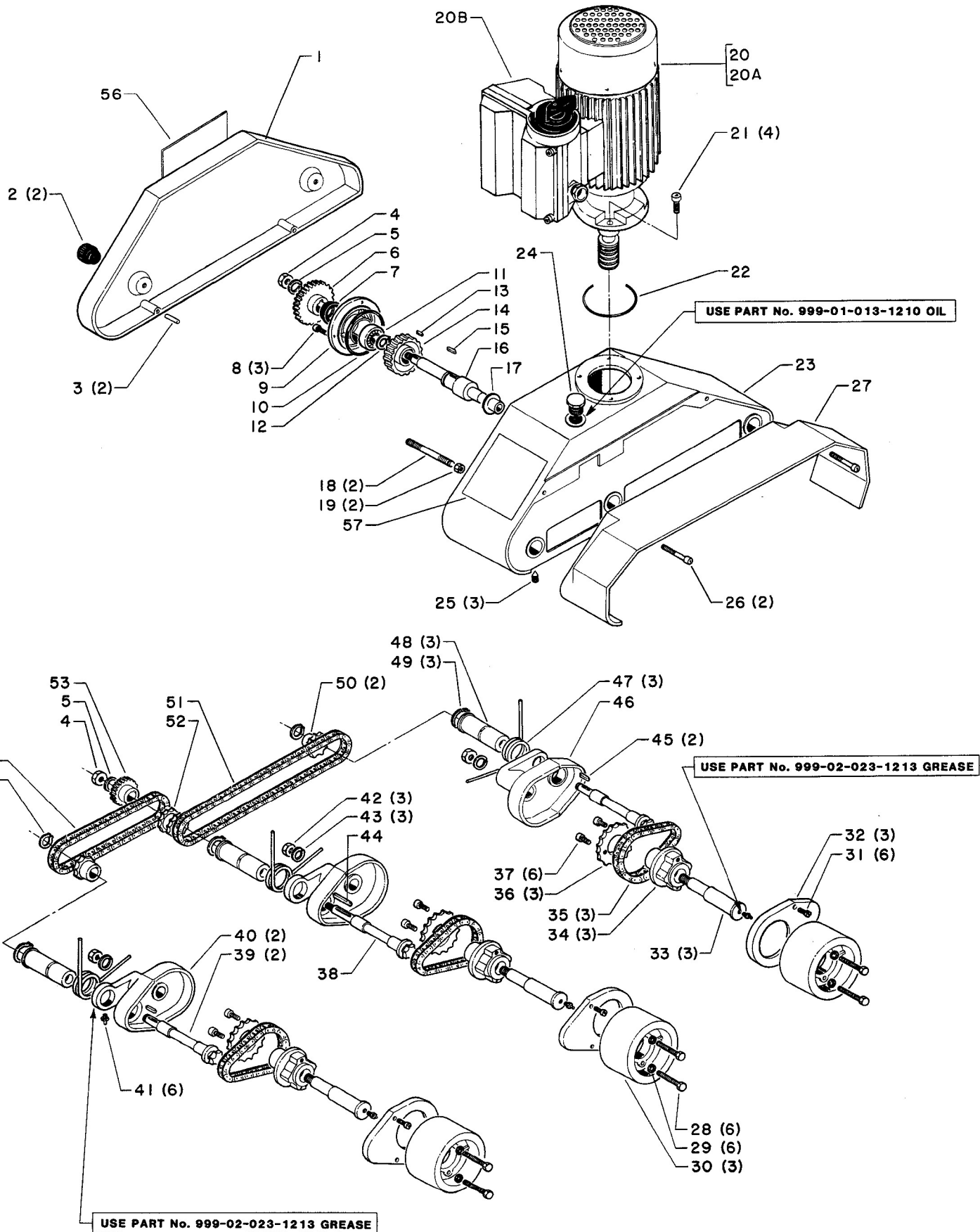
34-994 & 34-995 STOCKFEEDERS
