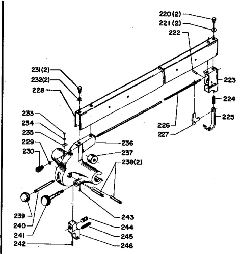
OLD STYLE RIP FENCE ASS'Y. 422-04-355-0001
