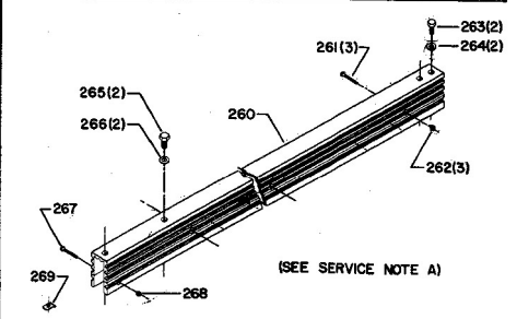
OLD STYLE TWO PIECE ALUMINUM RIP FENCE ASS'Y. EARLY 34-896
