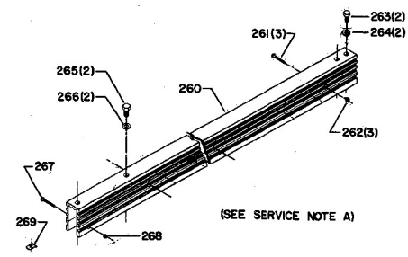
OLD STYLE TWO PIECE ALUMINUM RIP FENCE ASS'Y. EARLY 34-896
