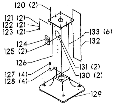
23-805 PEDESTAL EARLY MODELS ONLY
