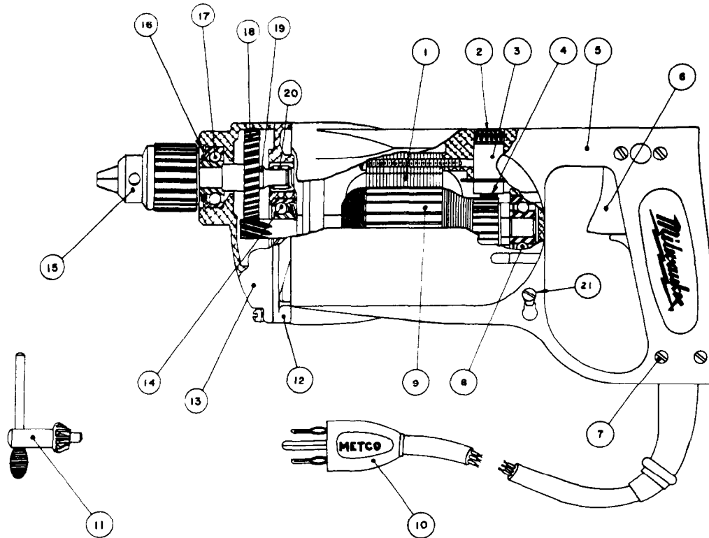
ILLUSTRATED PARTS
