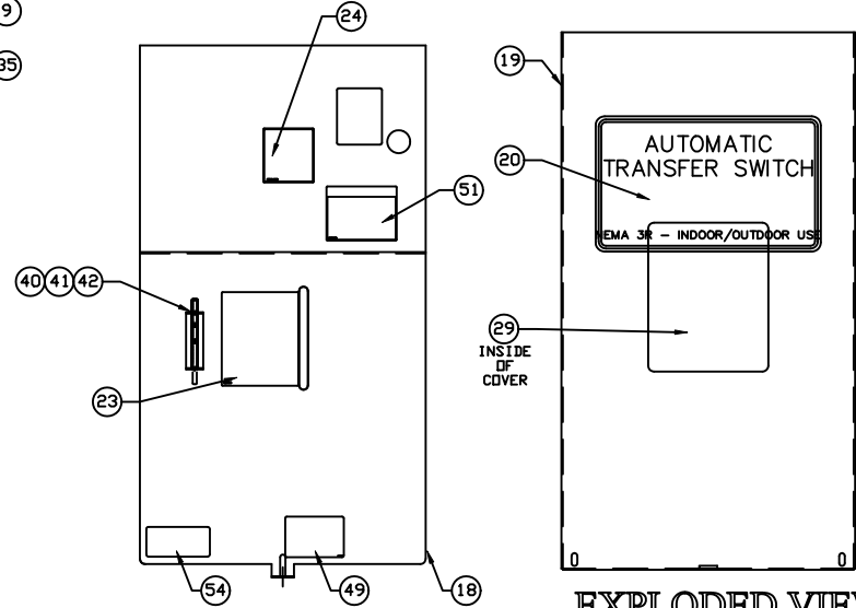
EXPLODED VIEW: 2-POLE TRANSFER SWITCH DRAWING #: 0E9801A
